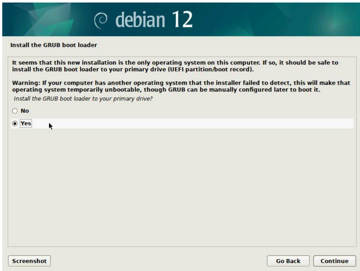
Installation: GRUB
