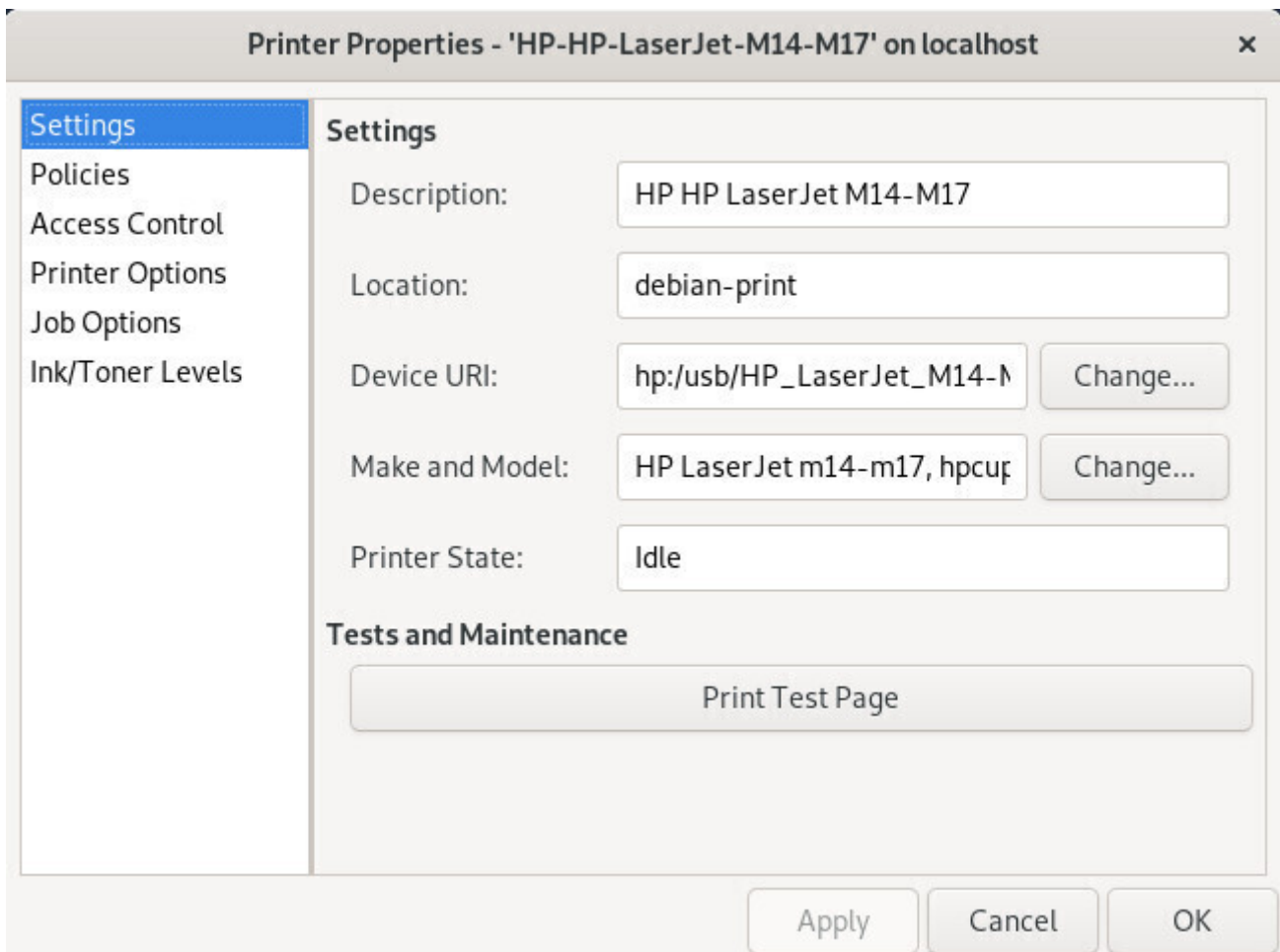
Printer configuration
