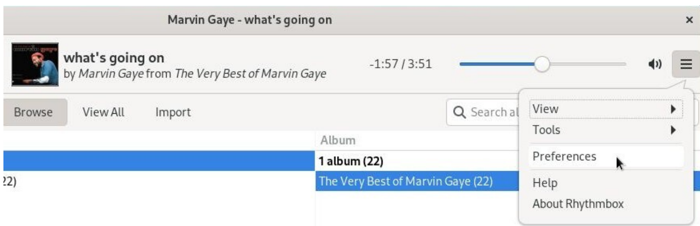
Rhythmbox: menu
