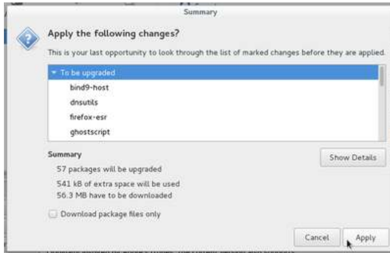
confirm changes
