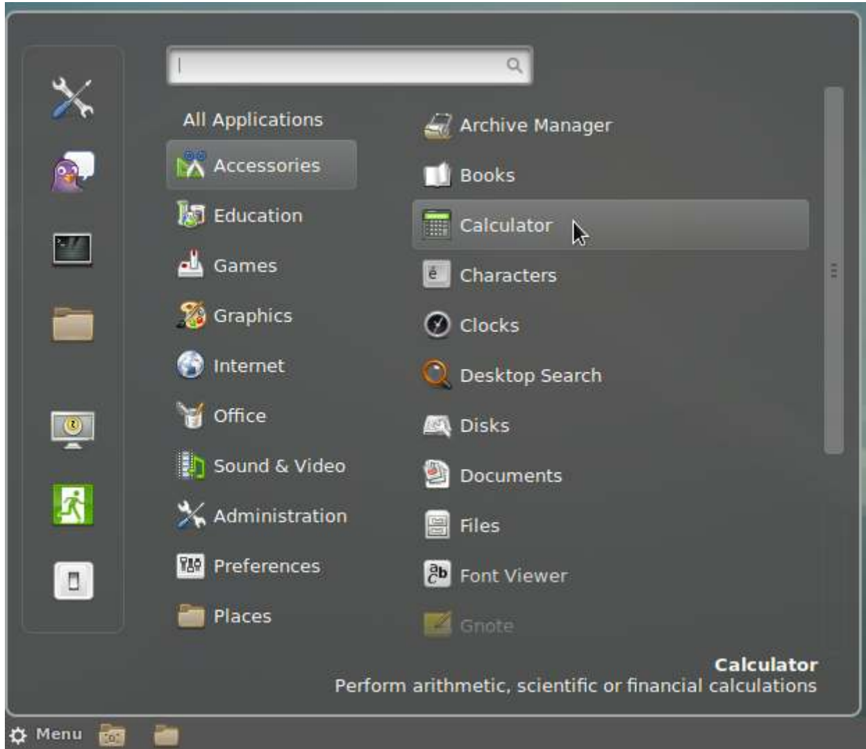
Cinnamon menu
