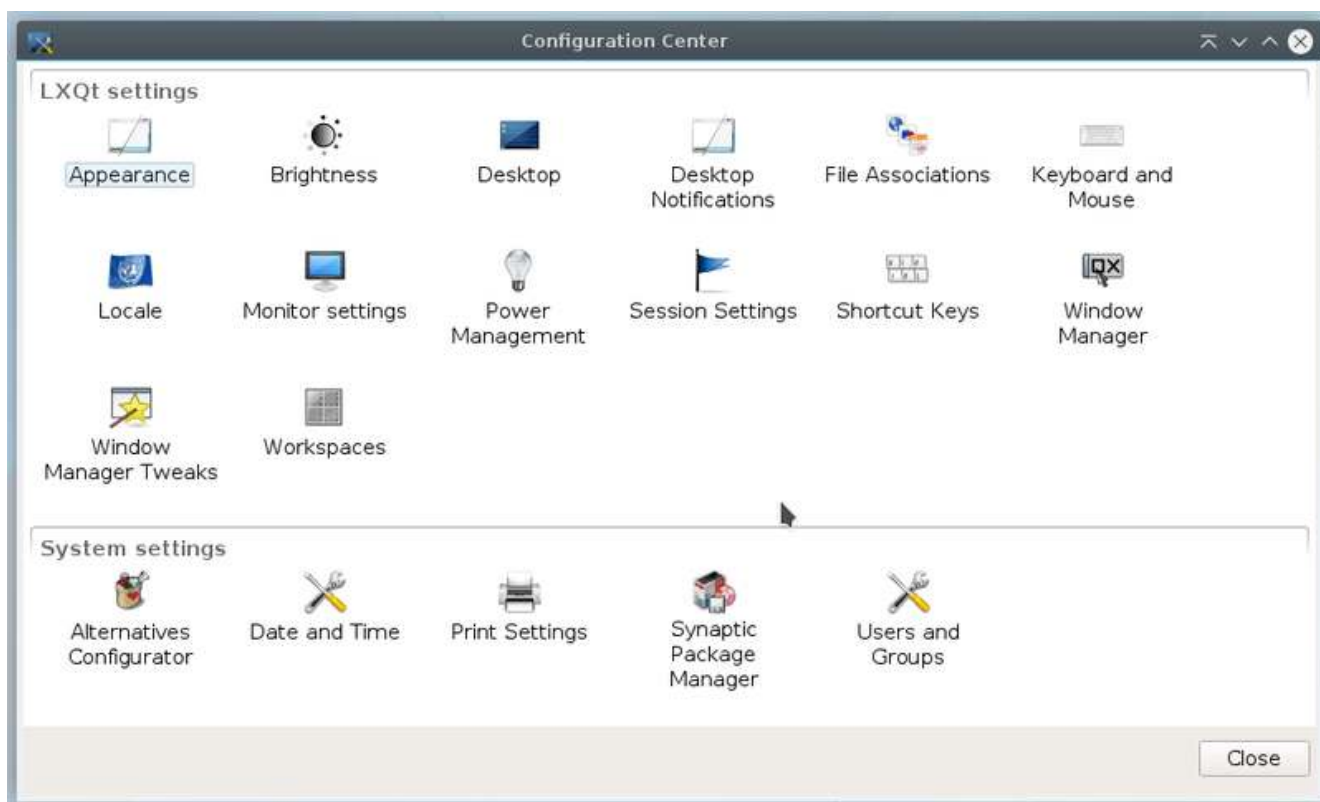
LXQt configuration
