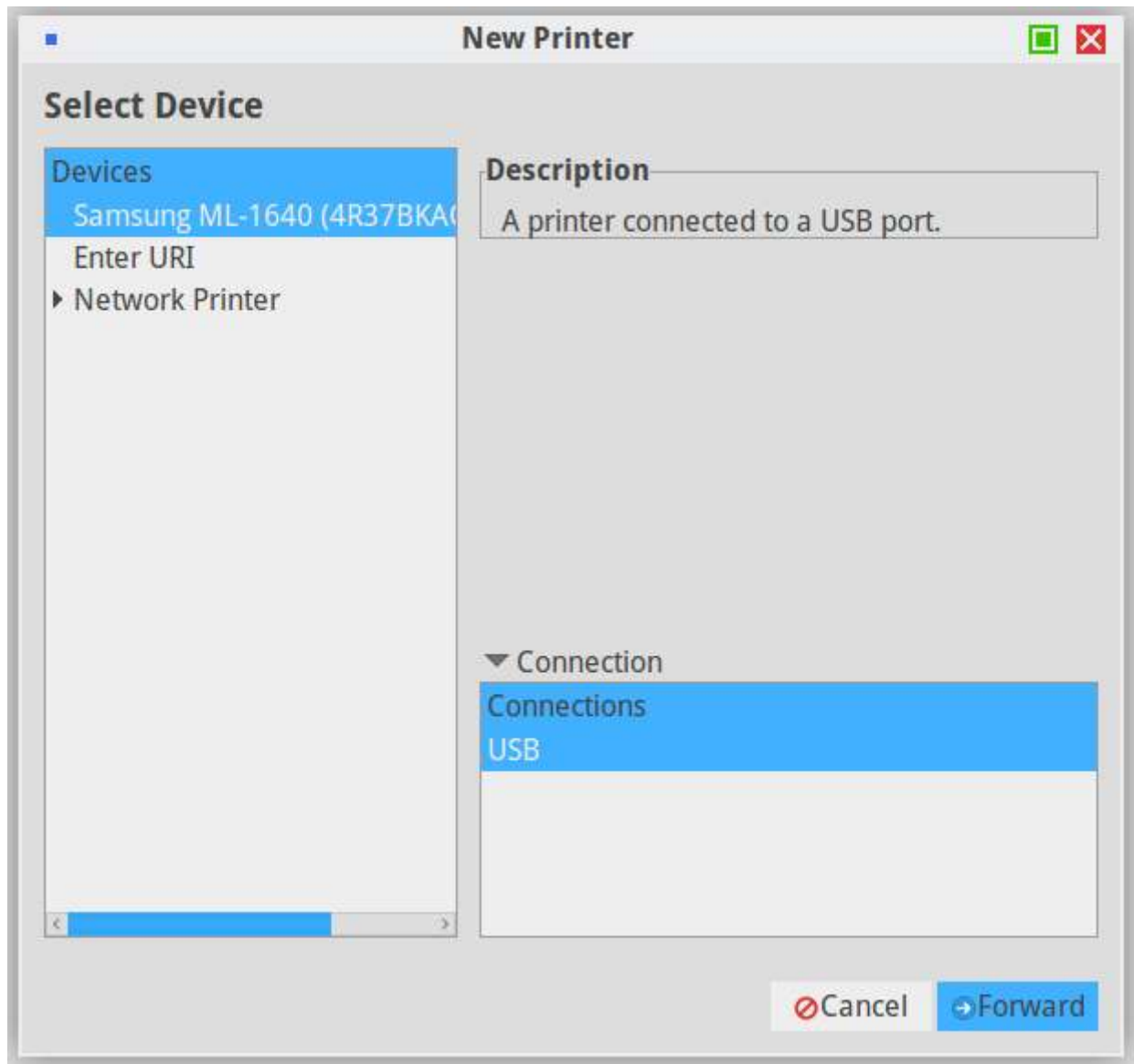
printer selection
