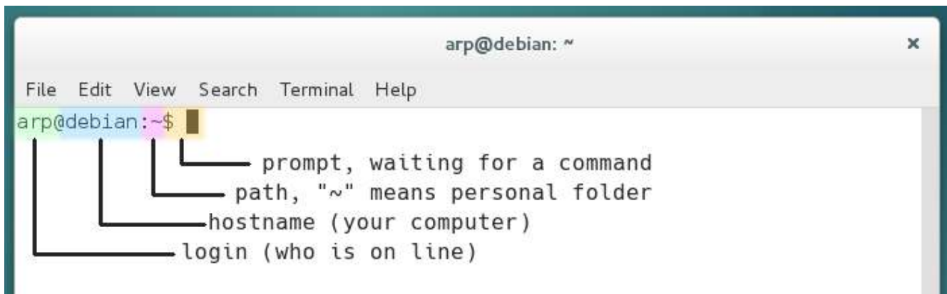
Terminal presentation
